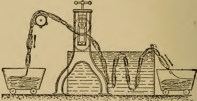
Fig. 156. WOOLEN CLOTH OPEN WIDTH SCOURING MACHINE.
